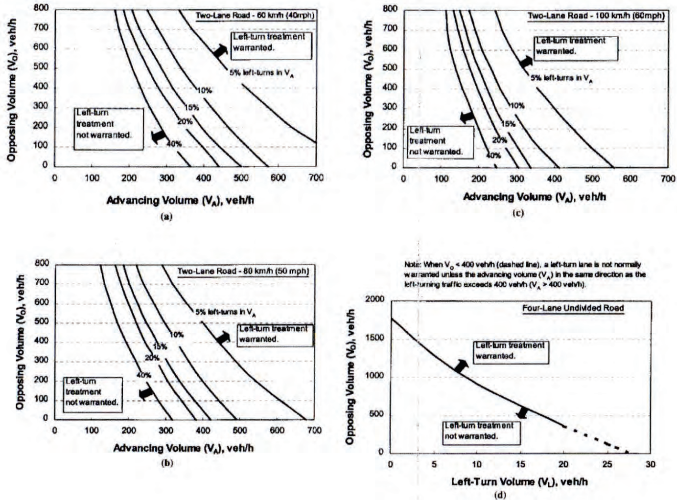
Figure 81 | Left-Turn Lane Warrants (Unsignalized Intersections) – Alternate Method
