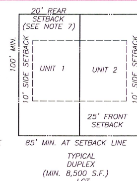
TYPICAL RESIDENTIAL LOTS N.T.S.
