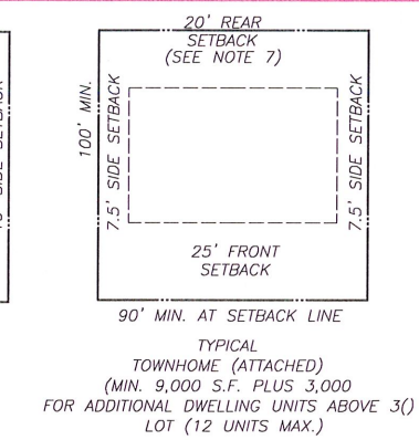
TYPICAL RESIDENTIAL LOTS N.T.S.
