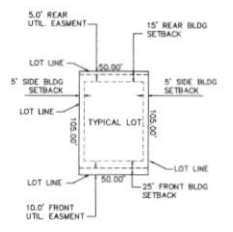
50' SINGLE FAMILY LOT N.T.S.
