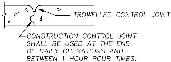
CONSTRUCTION CONTROL JOINT DETAIL
