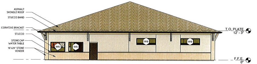
REAR ELEVATION 2 A.21 1/8" = 1'-0"
