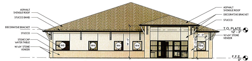
FRONT ELEVATION 4 A.21 1/8" = 1'-0"
