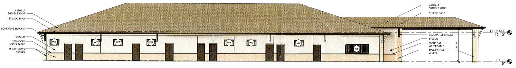
LEFT SIDE ELEVATION 1 A.21 1/8" = 1'-0"
