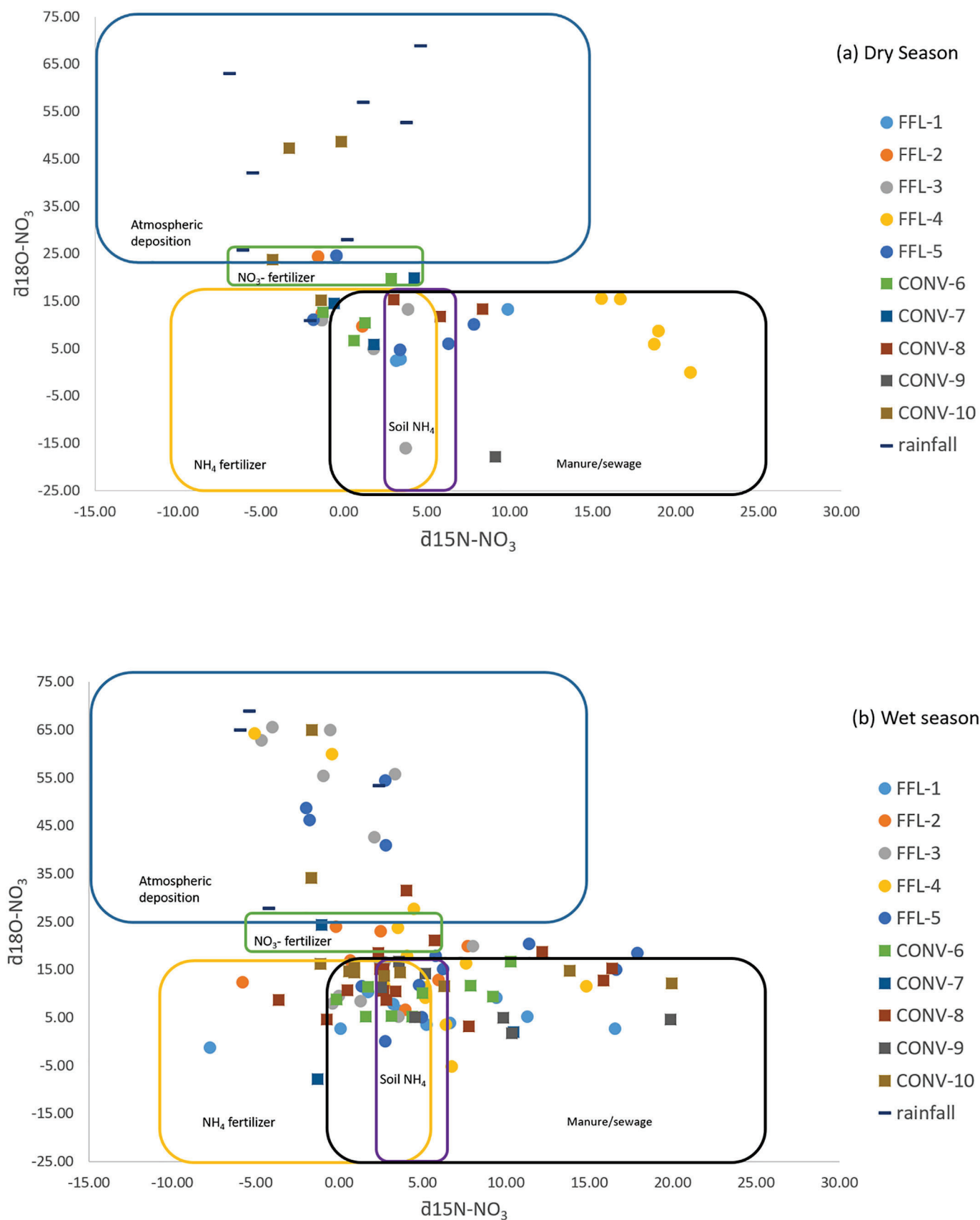
Fig. 5. Isotopic characterization of N and O in \text{NO}_3^- for rainfall and runoff samples in (a) dry season and (b) wet season.
