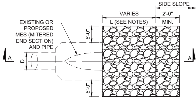
TYPICAL MES w/ RIPRAP RUBBLE
