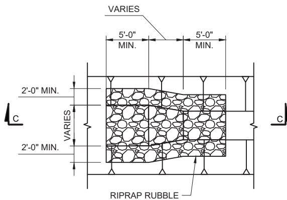
TYPICAL DITCH w/ RIPRAP RUBBLE
