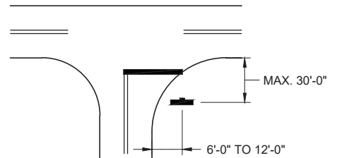
WIDE THROAT INTERSECTION
