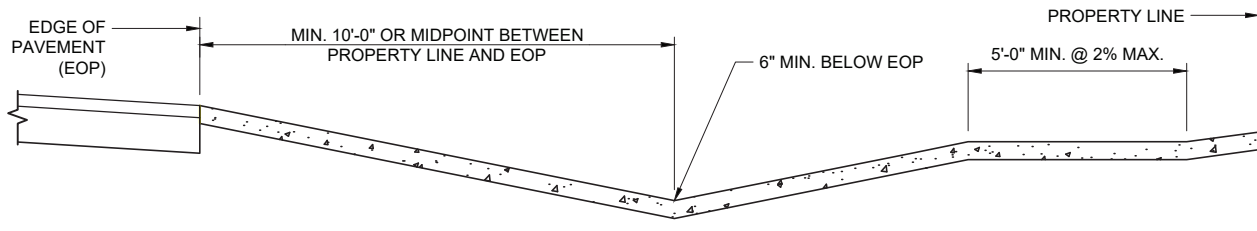
RESIDENTIAL CONNECTION SECTION WITHOUT CULVERT
