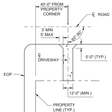
RESIDENTIAL DRIVEWAY PLAN - PAVED ROADS
