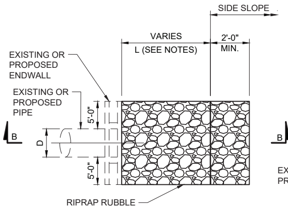
TYPICAL ENDWALL w/ RIPRAP RUBBLE
