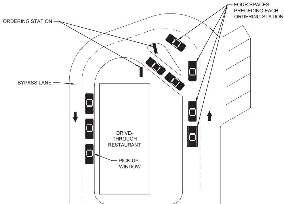
DUAL DRIVE THROUGH
