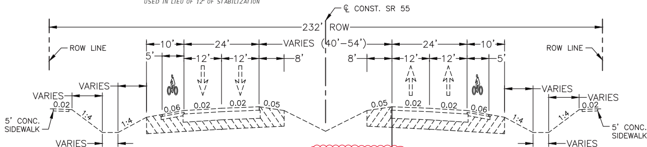
STATE ROAD 55 EXISTING TYPICAL SECTION STA 870+48.17 TO 1177+71.71 (LOOKING NORTH)
